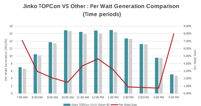
Figure 2: Time interval based per watt gain comparison
